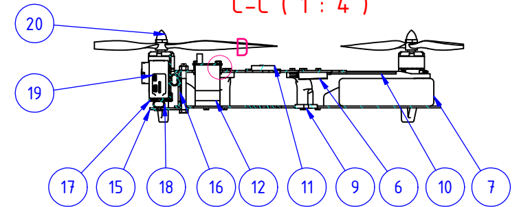
C-C (1:4)
